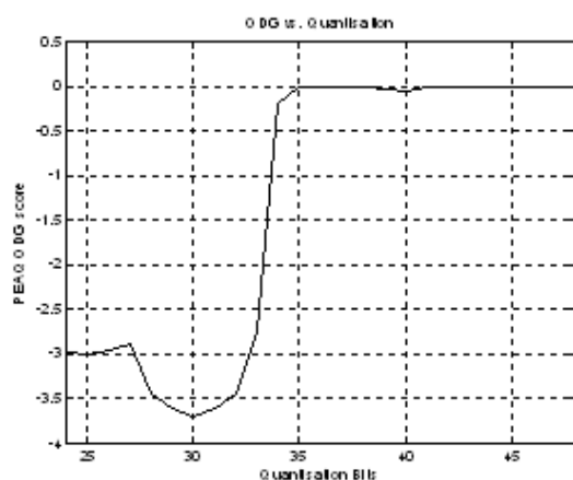
Fig. 11: ODG versus quantisation (E5 key)
