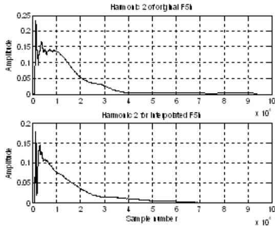
Fig. 9: Comparing 2 nd harmonic in COMB1
