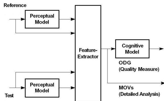
Fig. 7: Model for Perceptual Evaluation of Audio Quality (PEAQ)
