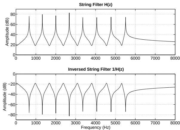
Fig. 6: Magnitude transfer function of string filter, key E5
