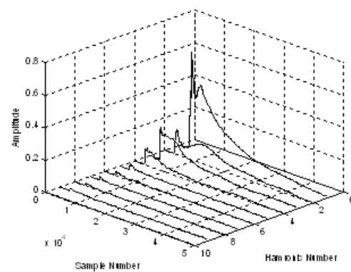
Fig. 3: Amplitude results of TEO
