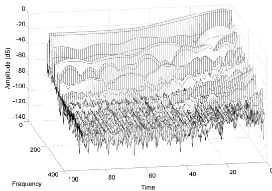
Fig. 2: Power spectrum of piano tone (key E5)
