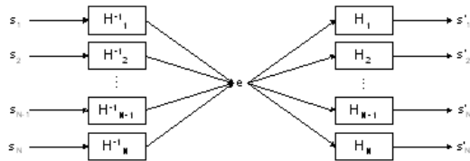
Fig. 5: Synthesis system of common excitation
